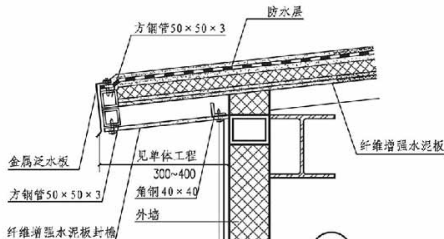
① 挑檐
