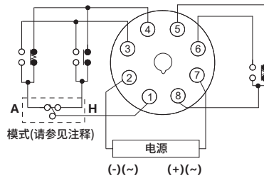
YEDH3BA-N8H (接点输出)
