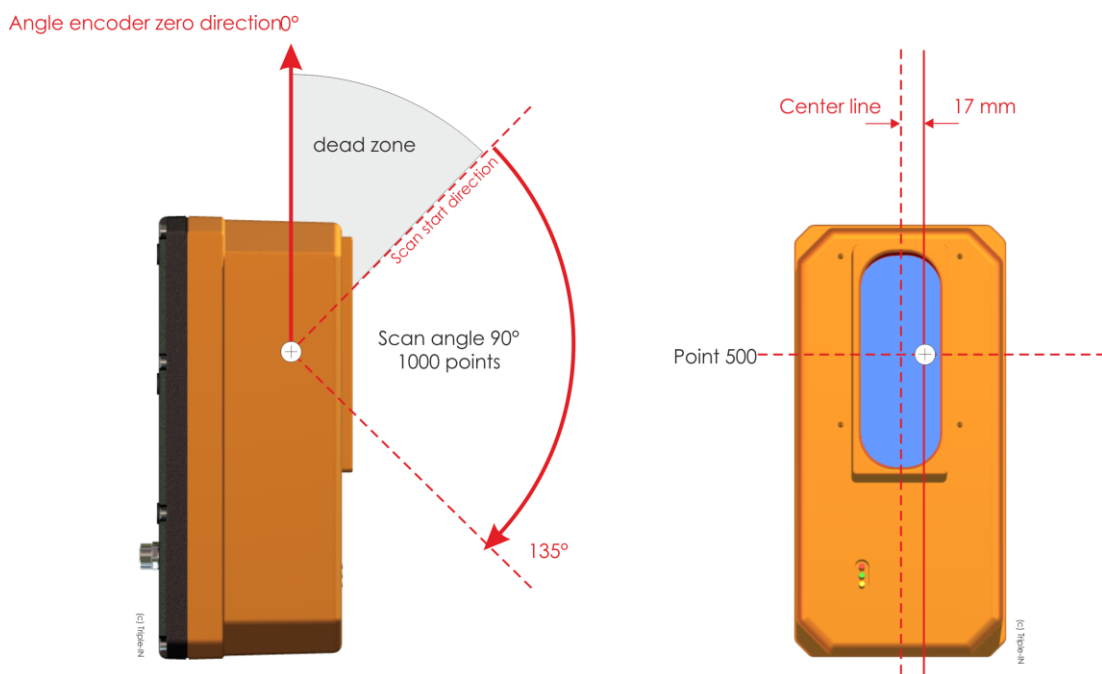
Figure 6: PAC250-90-y-zz+ Laser Scanners scan area and point of origin
