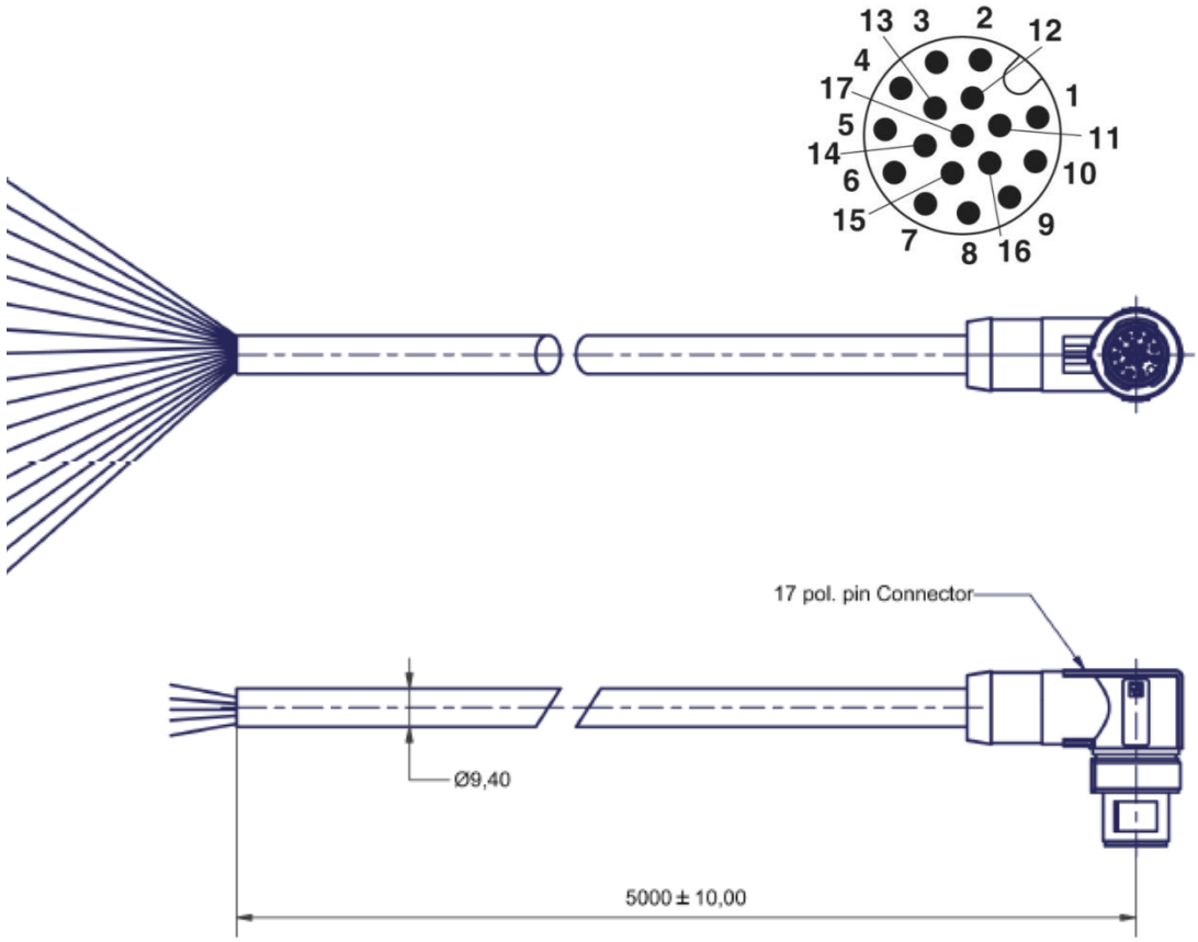
Figure 48: Multifunction cable
