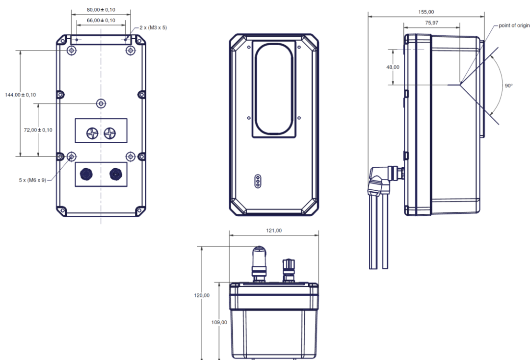
Figure 47: PAC250-90-y-zz+ Laser Scanners outlines (no scale)
