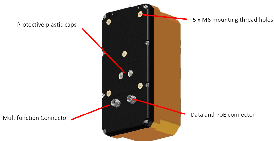
Figure 5: PAC250-90-y-zz+ Laser Scanners rear side
