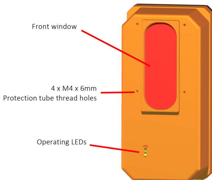
Figure 4: PAC250-90-y-zz+ Laser Scanners front side
